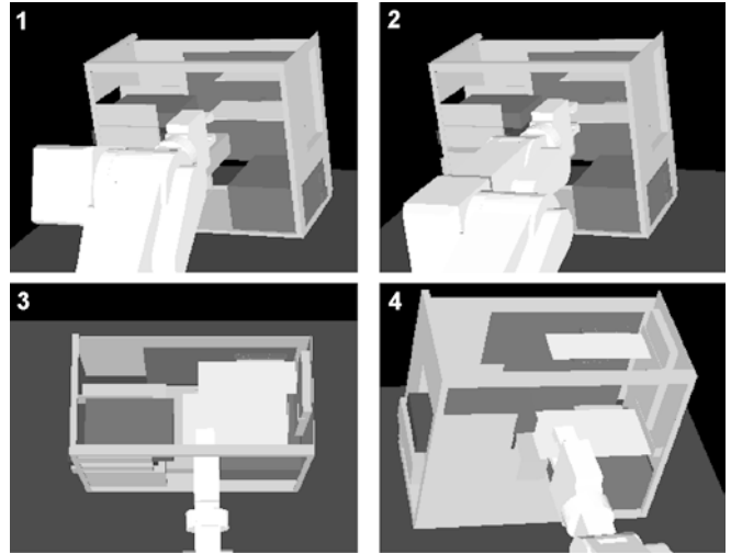
Fig. 8 Photographs of simulation sequence for disassembly trajectory of the component “video card” from different view points
